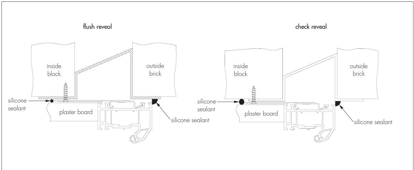
Figure 3 Typical head with window detail
