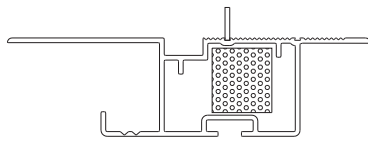
WF39036 90 mm cavity — jamb
