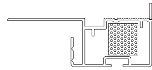
WF37546 75 mm cavity — jamb in-check
