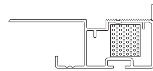
WF39046 90 mm cavity — jamb in-check
