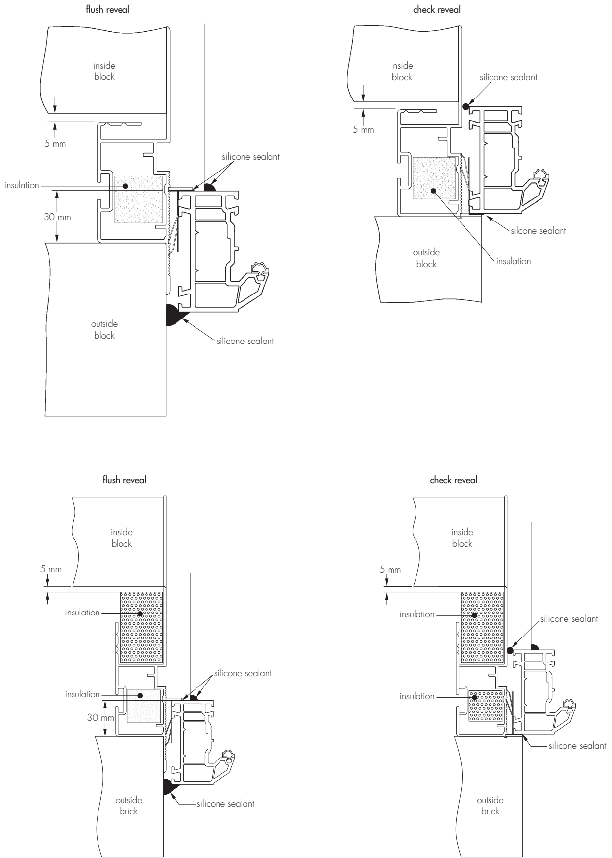
Figure 4 Typical jamb with window detail
