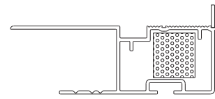
WF31046 100 mm cavity — jamb in-check
