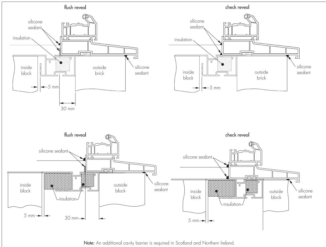
Figure 5 Typical sill with window detail
