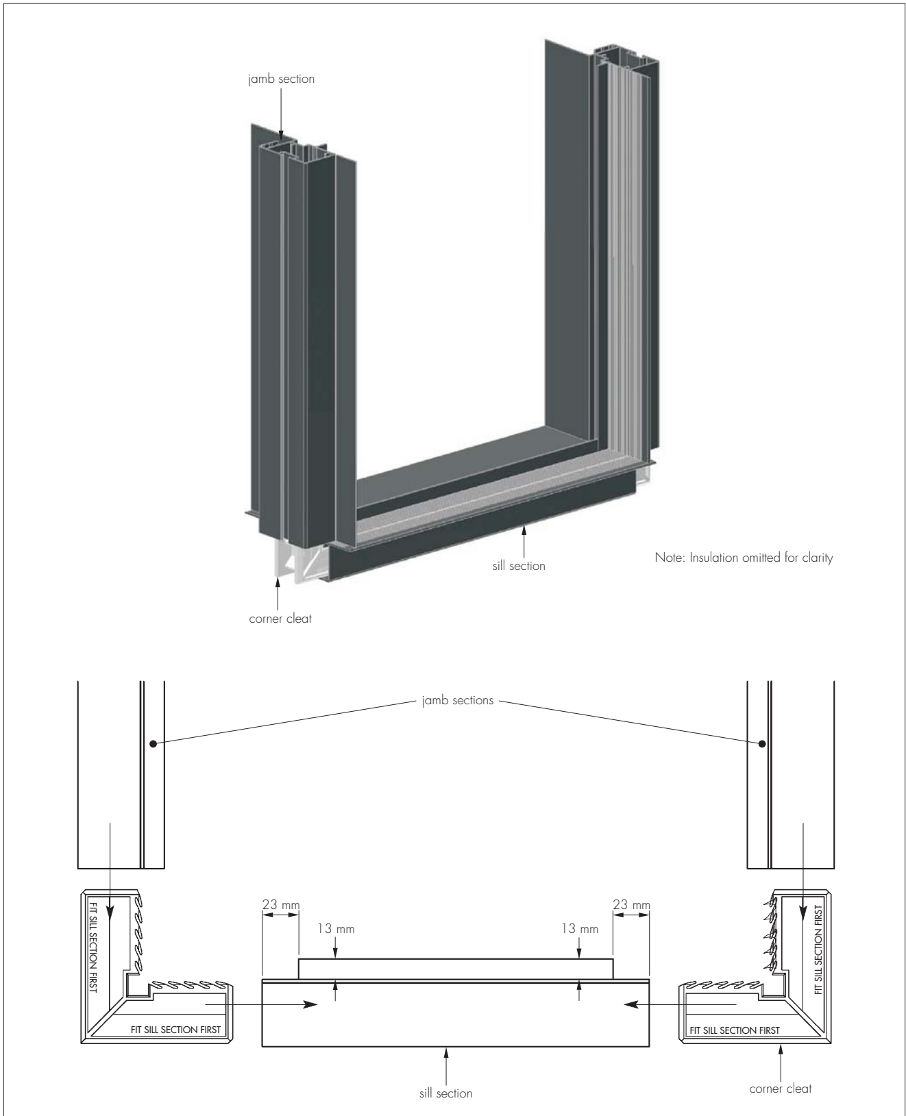
Figure 2 Winfit sub-frame fabrication
