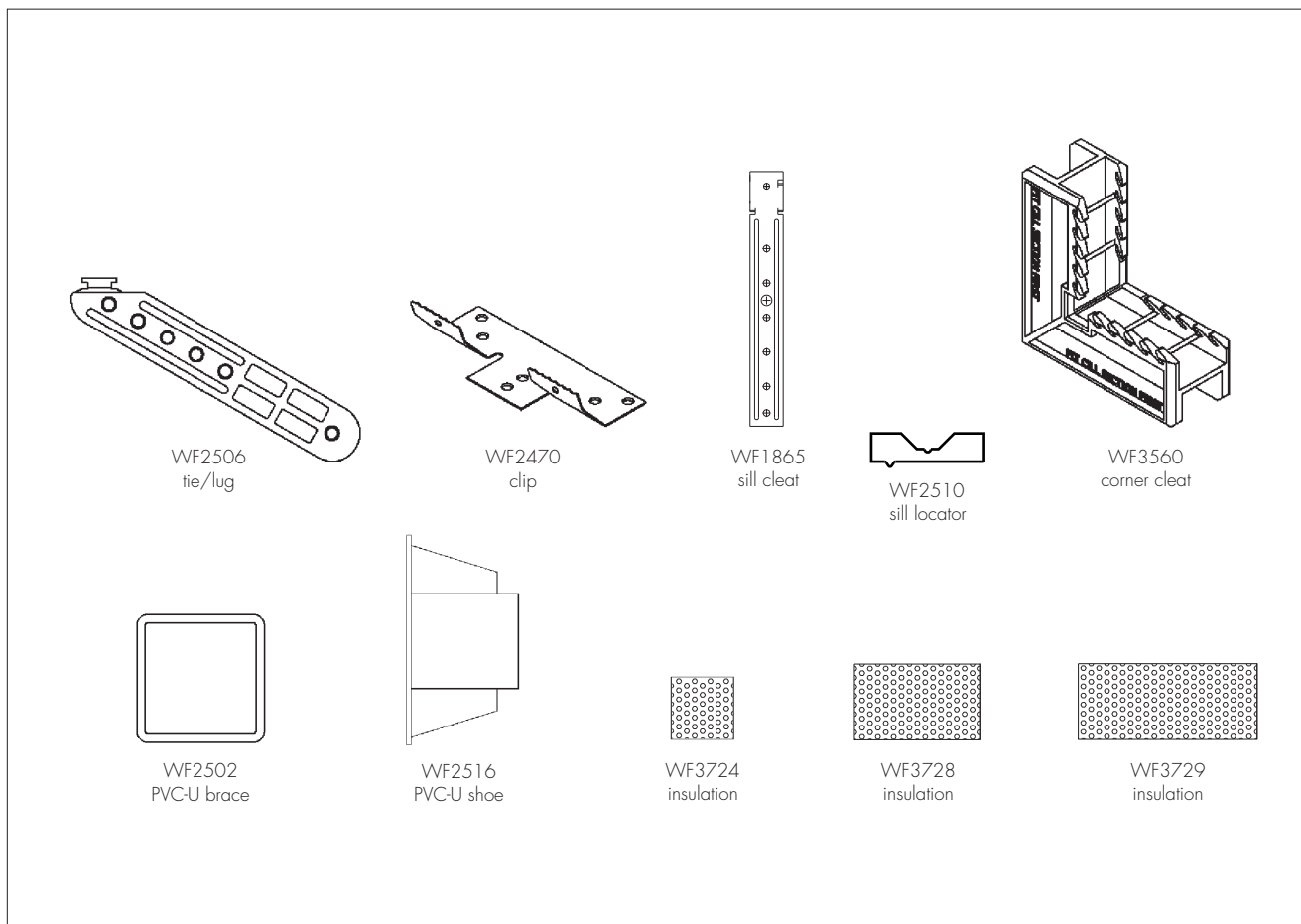
Figure 1 Winfit components (continued)
