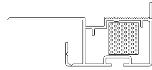
WF38046 80 mm cavity — jamb in-check
