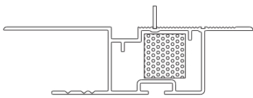
WF31036 100 mm cavity — jamb
