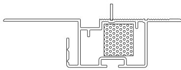
WF37536 75 mm cavity — jamb
